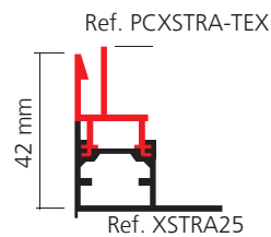
XSTRA 25 TEXTILE simple face
